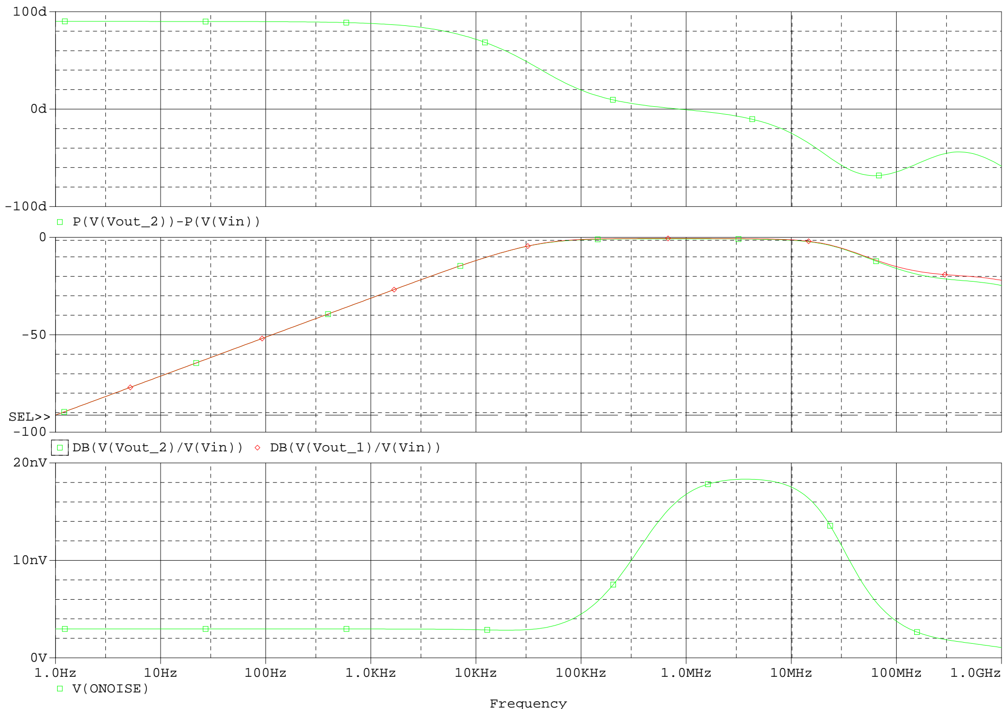
(A) AC sweep.dat (active)
