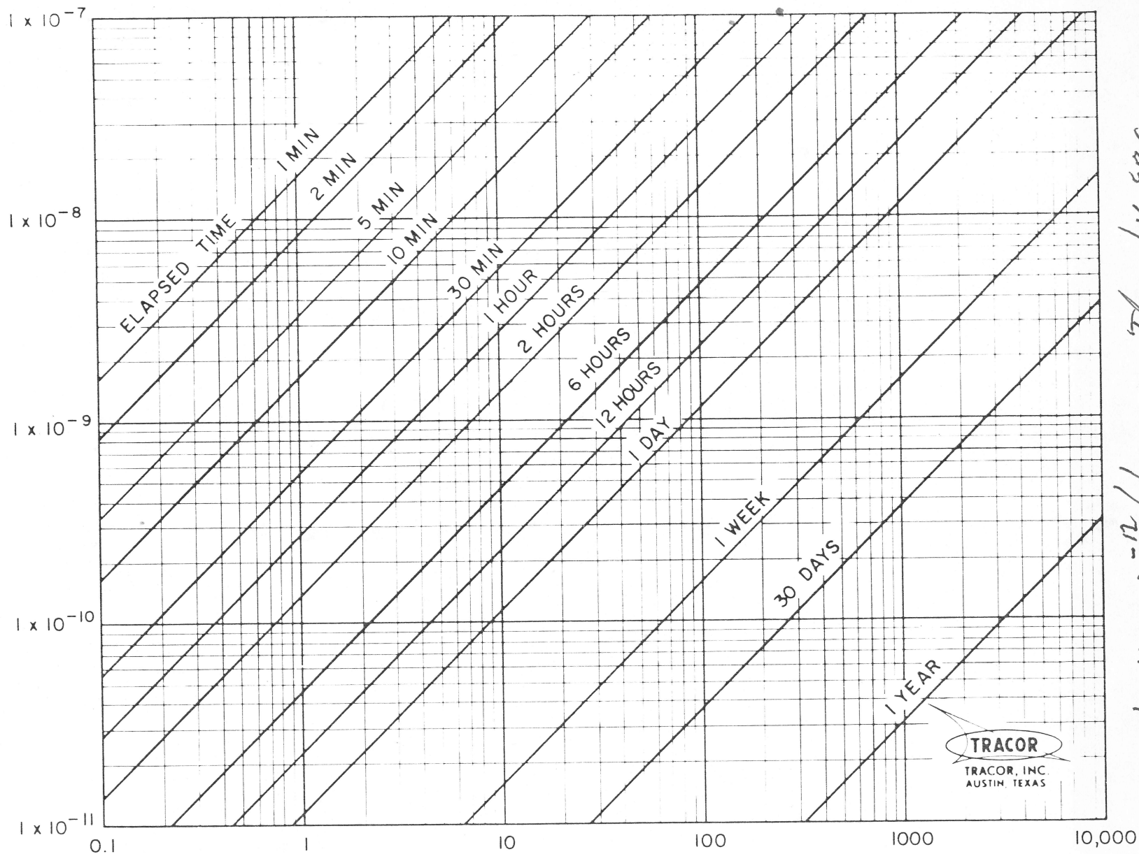
Figure 5-1. ACCUMULATED TIME ERROR, MICROSECONDS
