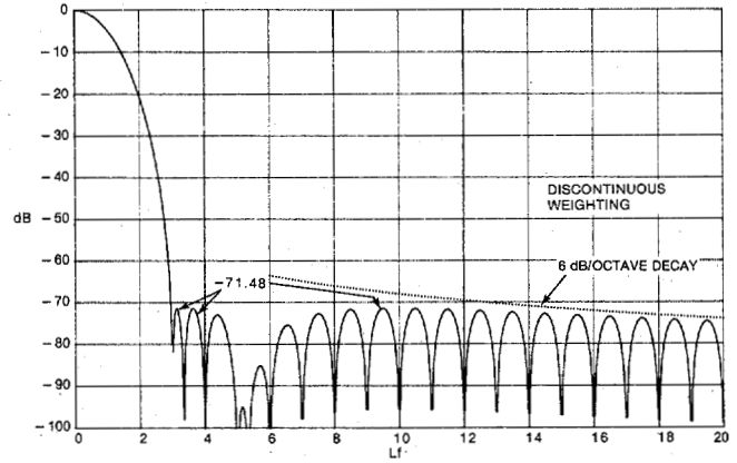
Fig. 14. Minimum 3-term window for a_0 = 0.4243801 , a_1 = 0.4973406 , a_2 = 0.0782793 .
