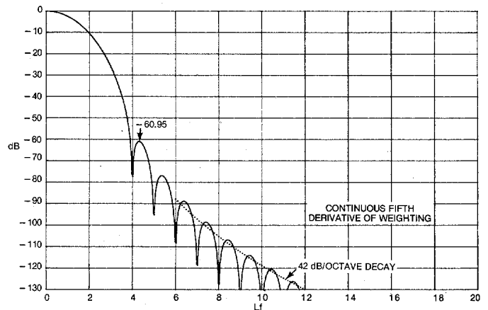
Fig. 10. Window for a_0 = 10/32 , a_1 = 15/32 , a_2 = 6/32 , a_3 = 1/32 .
