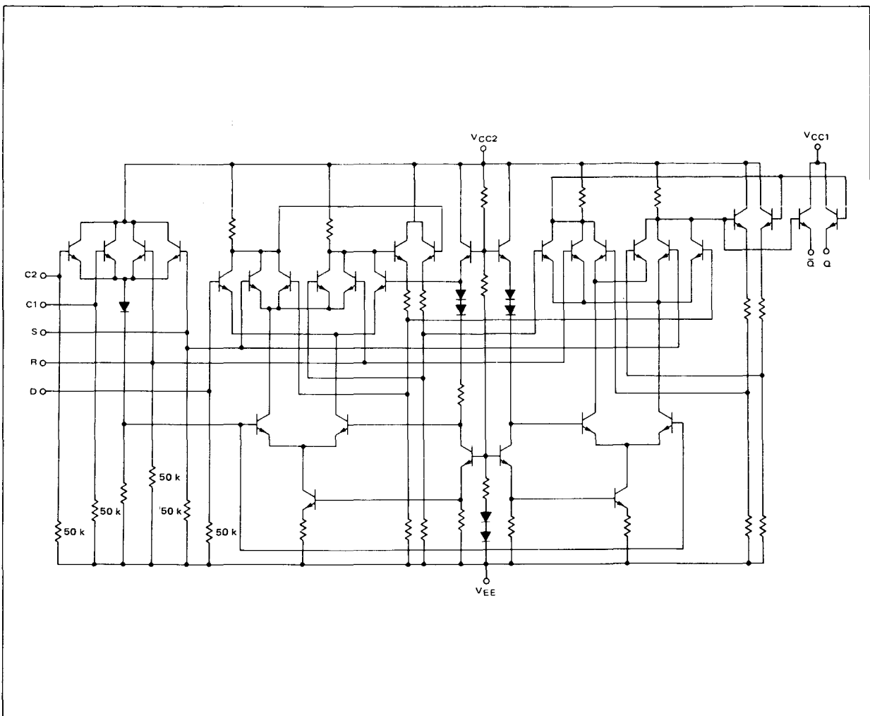
FIGURE 10 – MC1670 CIRCUIT SCHEMATIC
