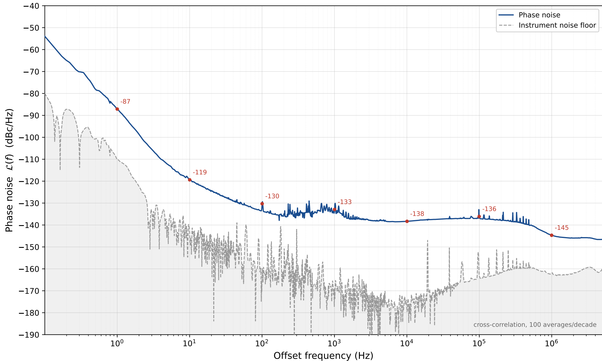
8663a-Phase noise — 10 MHz carrier
